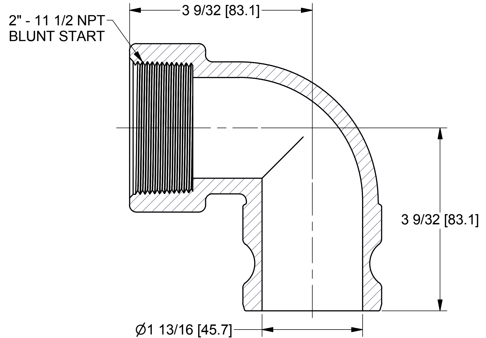
SECTION B-B SCALE 1 : 1
